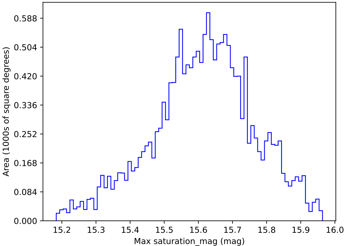
too_100_1v3.4_10yrs WFD i band: Max saturation_mag
