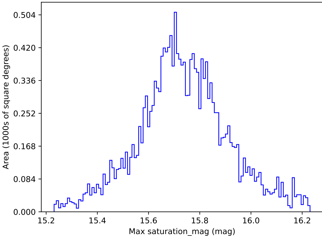
too_100_1v3.4_10yrs WFD g band: Max saturation_mag
