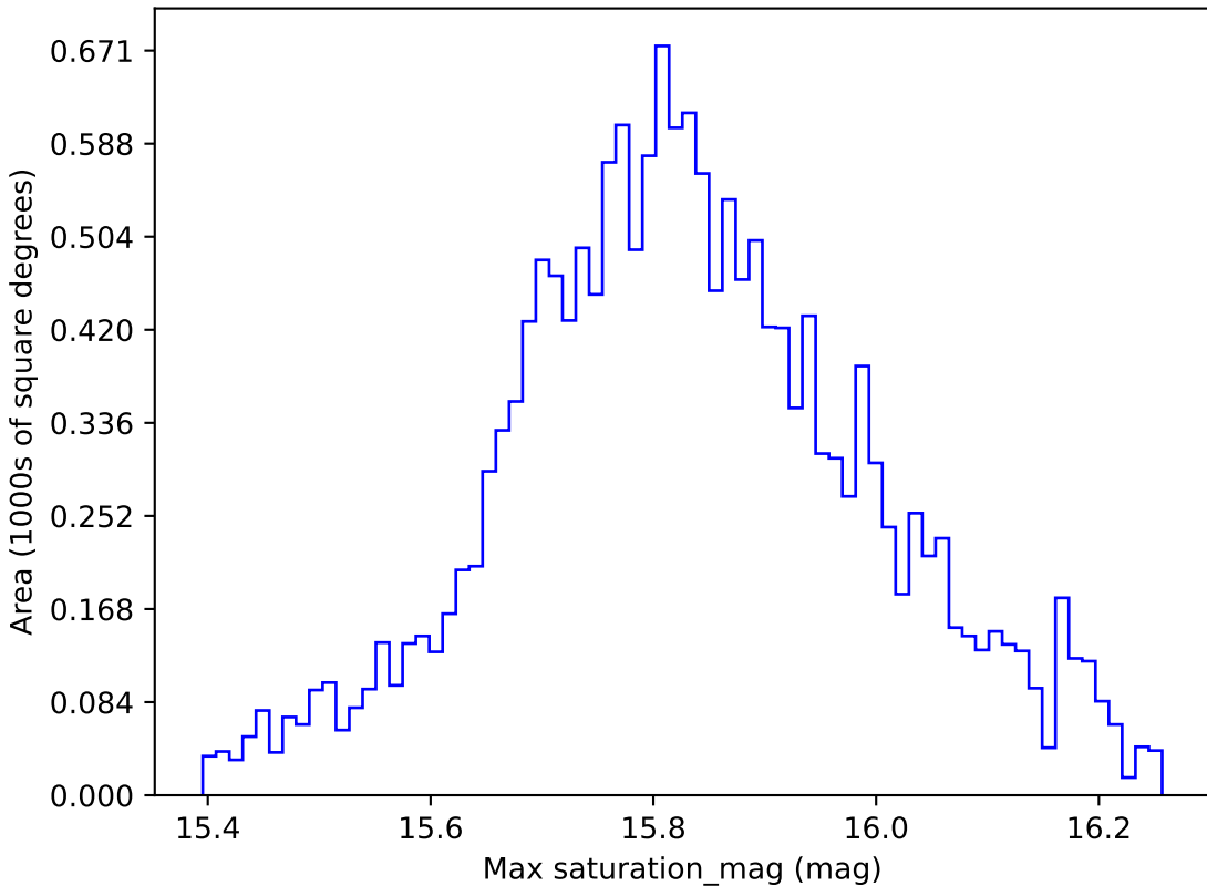
too_100_1v3.4_10yrs WFD all bands: Max saturation_mag
