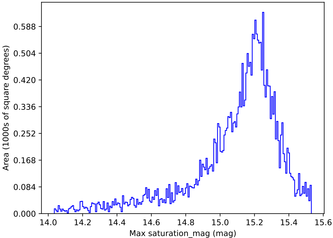
too_100_1v3.4_10yrs All sky z band: Max saturation_mag
