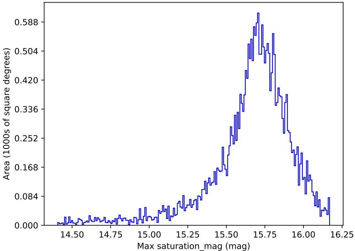
too_100_1v3.4_10yrs All sky r band: Max saturation_mag
