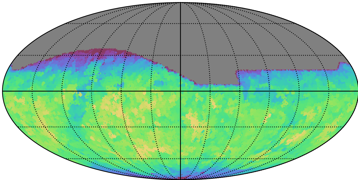
too_100_1v3.4_10yrs All sky i band: Max saturation_mag
