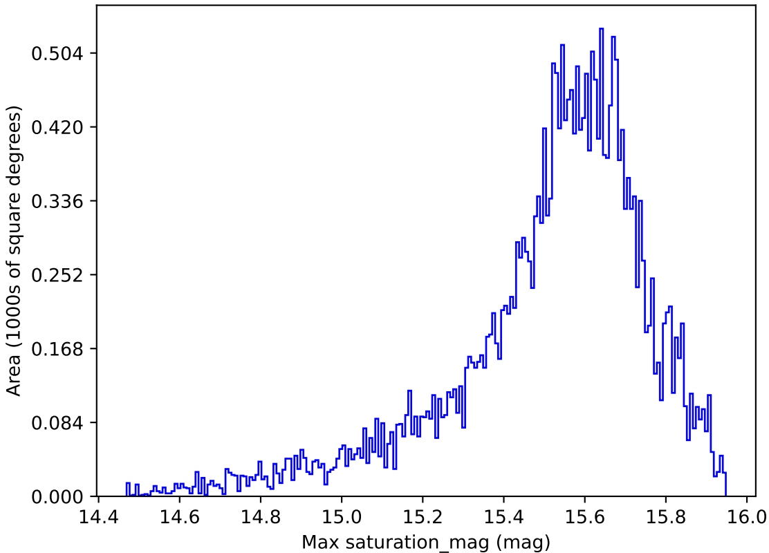
too_100_1v3.4_10yrs All sky i band: Max saturation_mag
