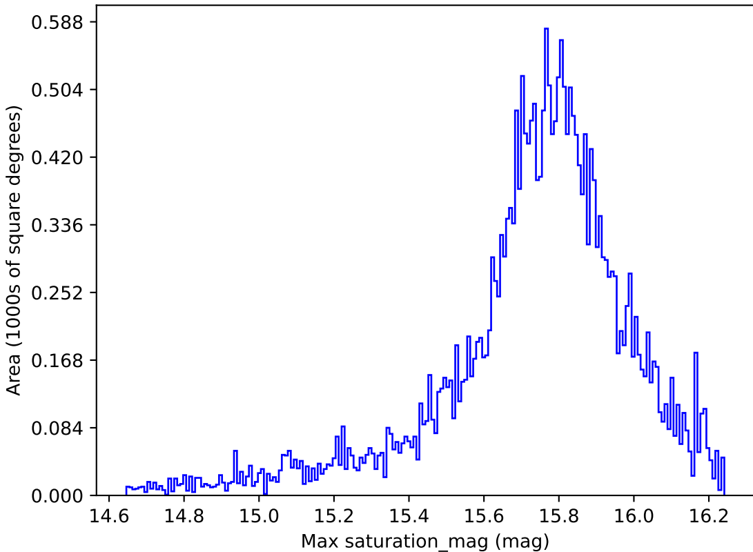
too_100_1v3.4_10yrs All sky all bands: Max saturation_mag
