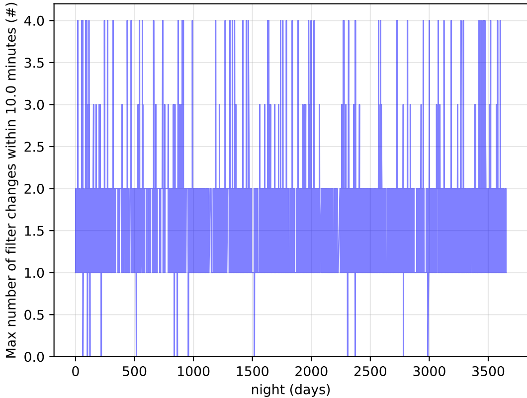
too_100_1v3.4_10yrs Per Night: Max number of filter changes within 10.0 minutes
