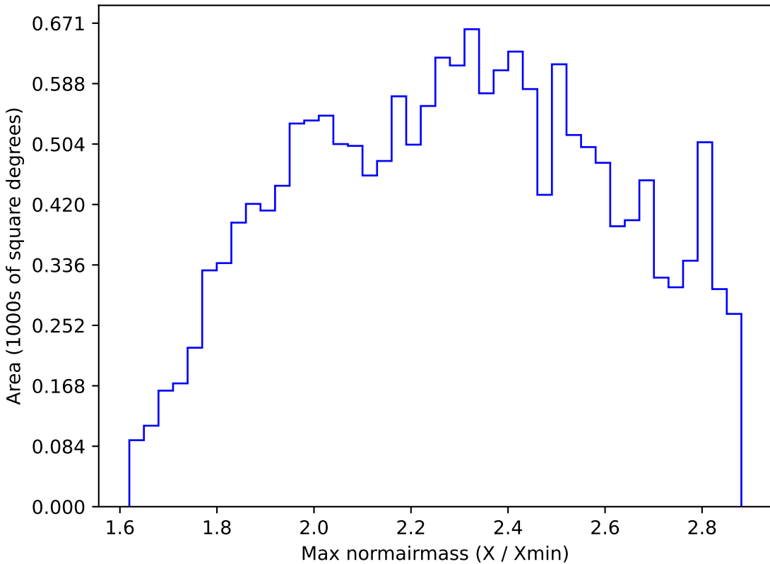
too_100_1v3.4_10yrs WFD z band: Max normairmass
