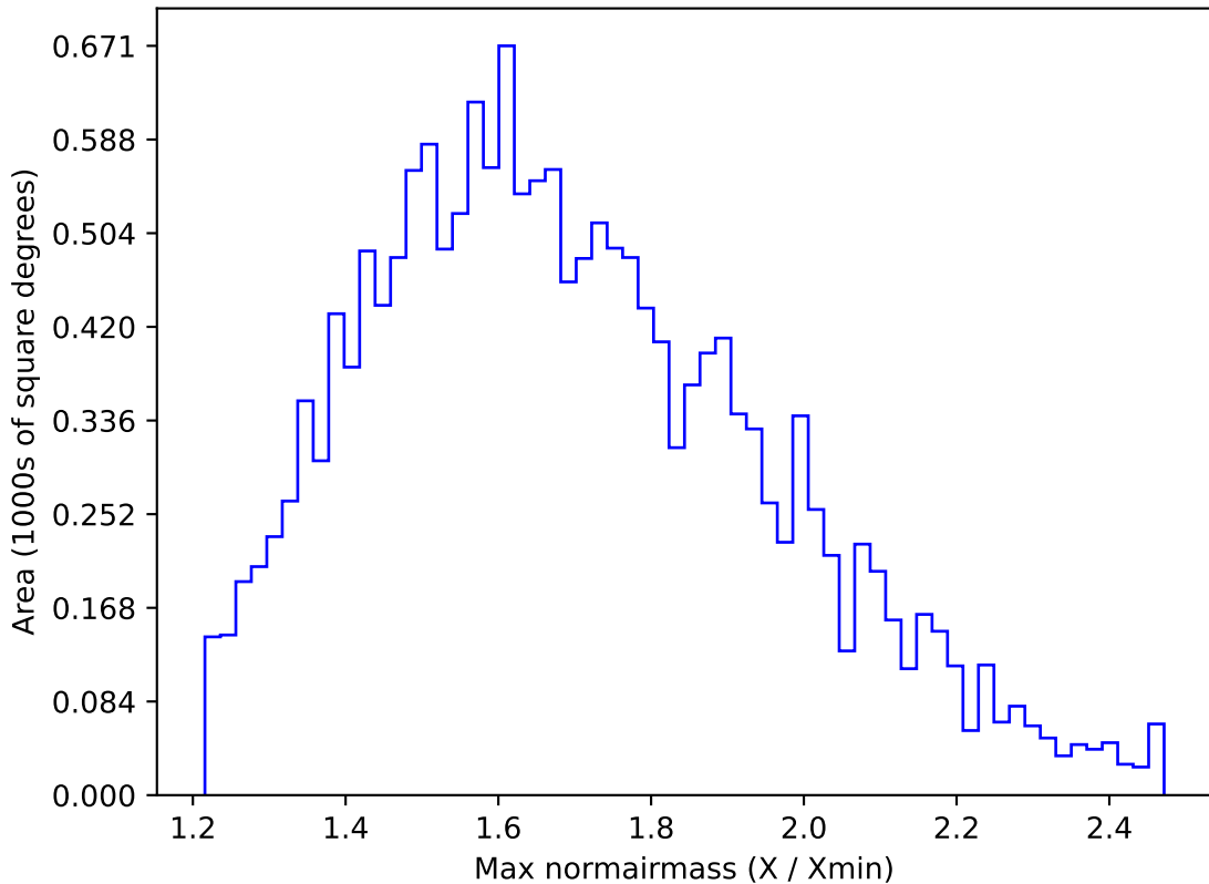
too_100_1v3.4_10yrs WFD u band: Max normairmass
