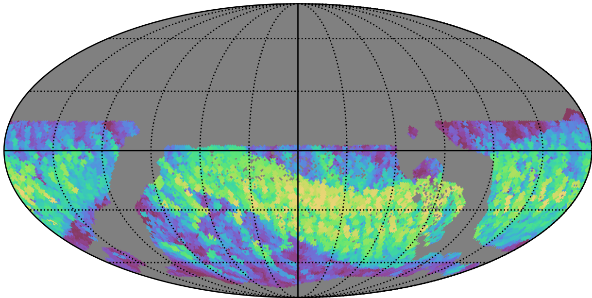
too_100_1v3.4_10yrs WFD i band: Max normairmass
