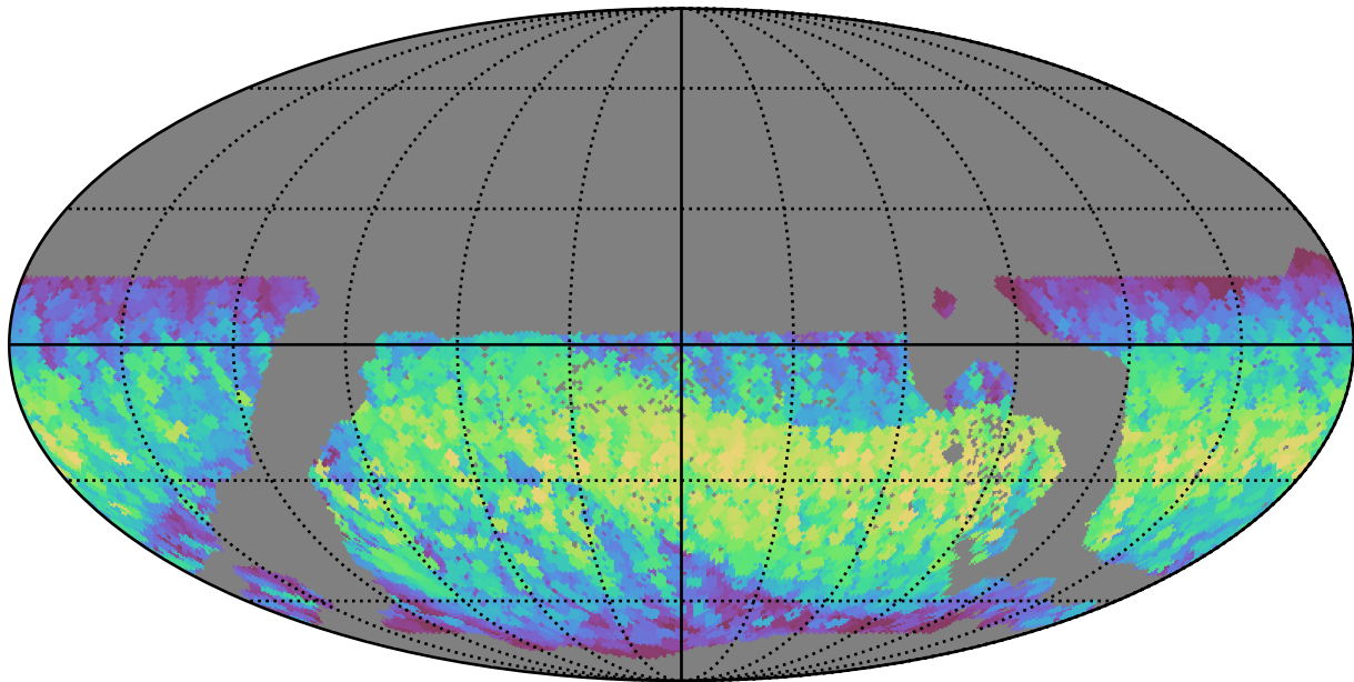
too_100_1v3.4_10yrs WFD all bands: Max normairmass
