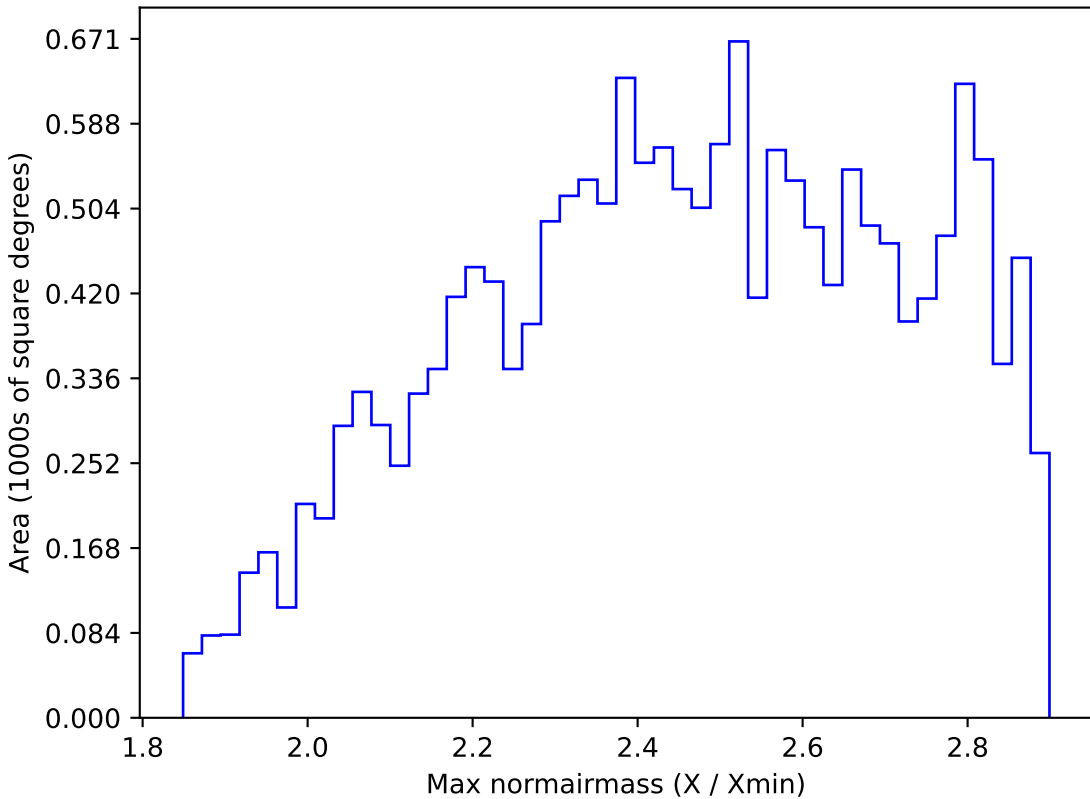
too_100_1v3.4_10yrs WFD all bands: Max normairmass
