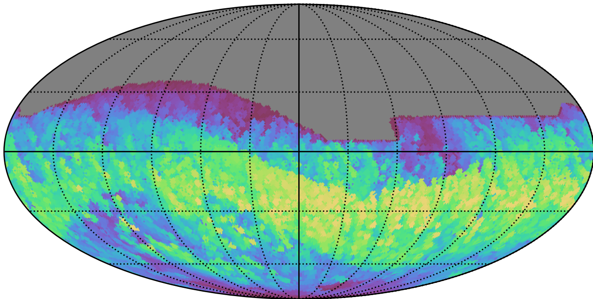
too_100_1v3.4_10yrs All sky z band: Max normairmass
