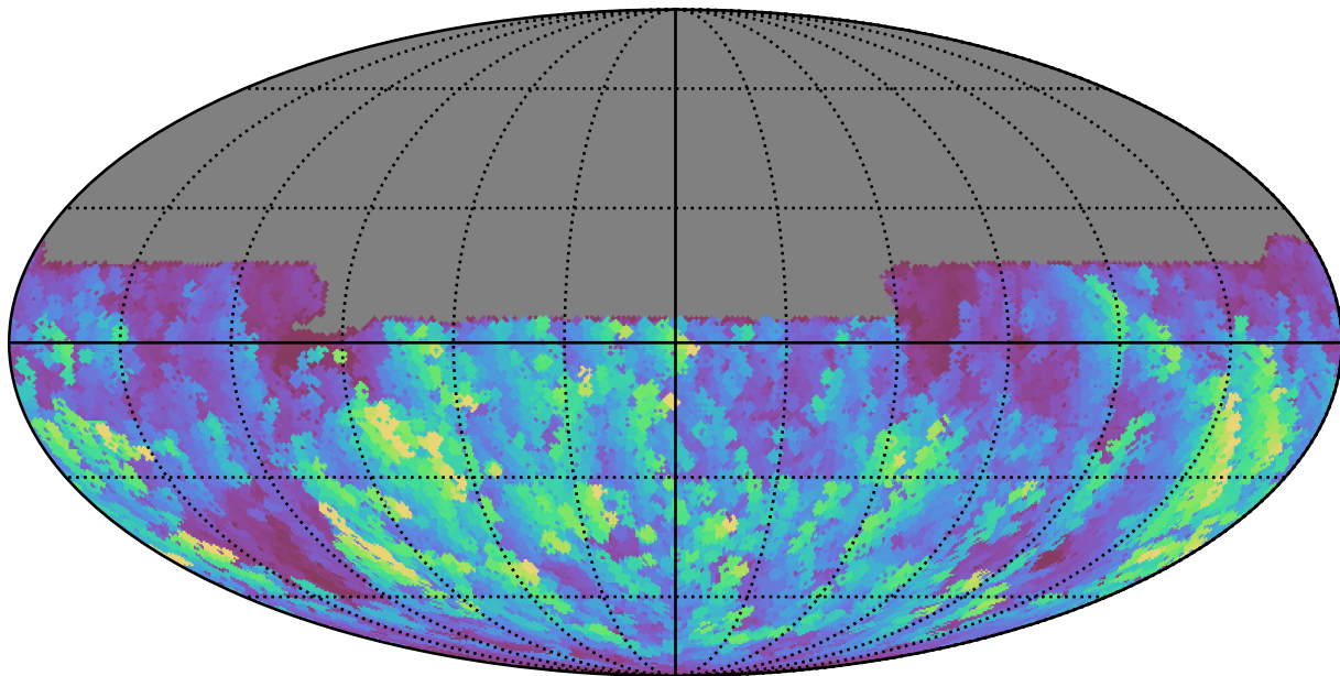
too_100_1v3.4_10yrs All sky u band: Max normairmass
