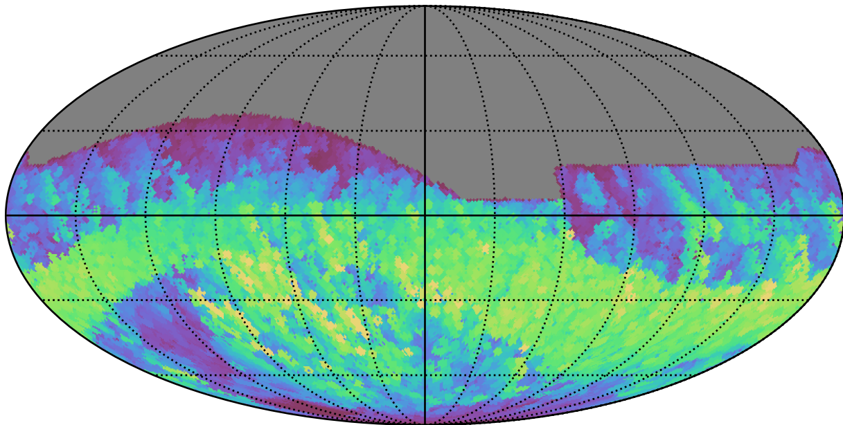
too_100_1v3.4_10yrs All sky r band: Max normairmass
