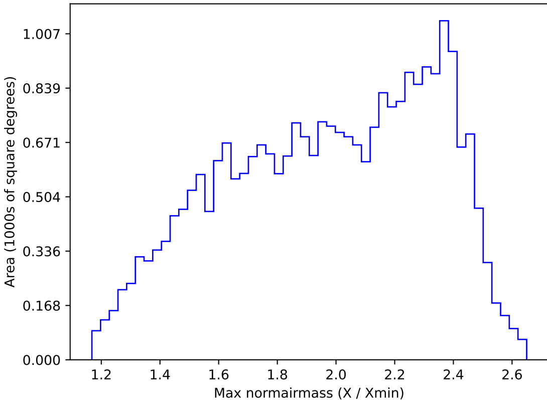
too_100_1v3.4_10yrs All sky r band: Max normairmass
