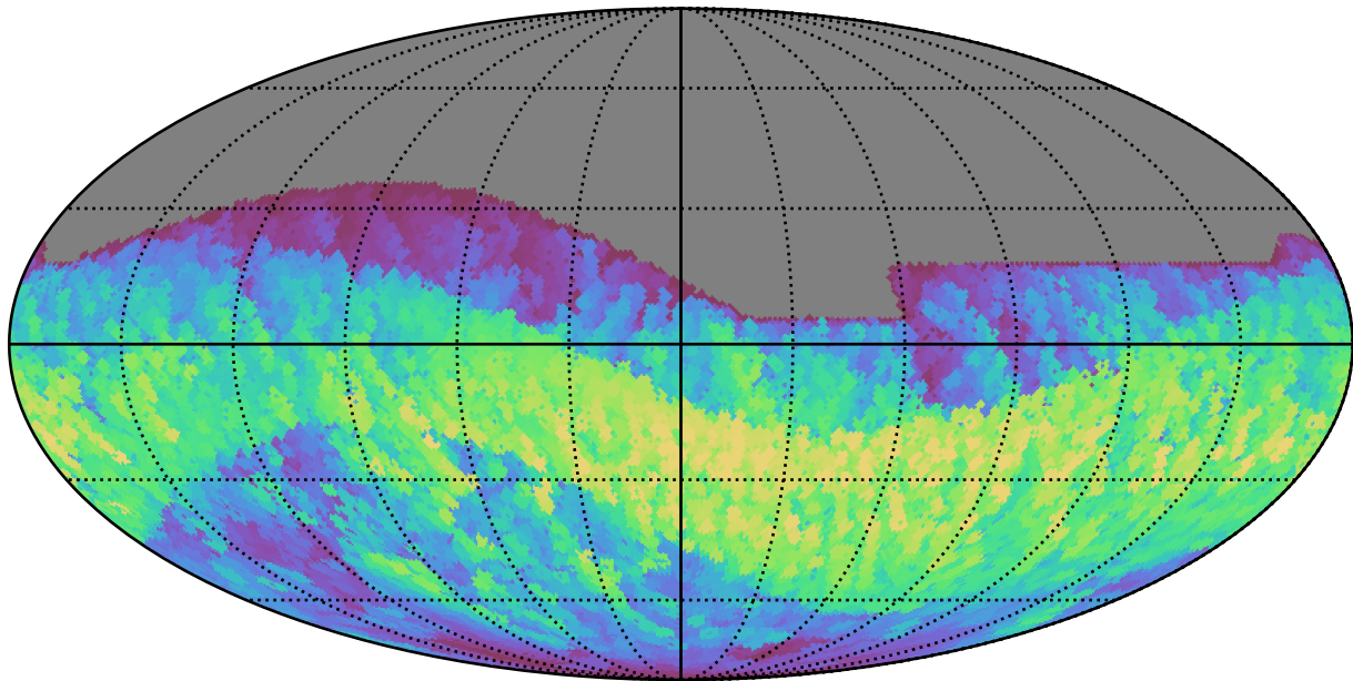
too_100_1v3.4_10yrs All sky i band: Max normairmass
