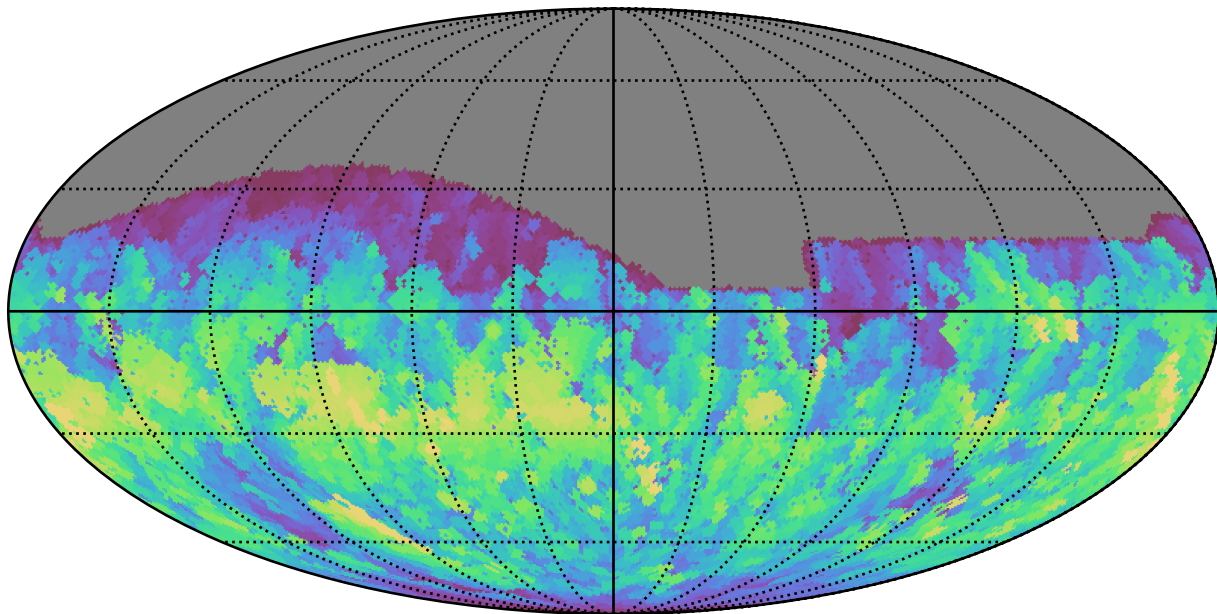
too_100_1v3.4_10yrs All sky g band: Max normairmass
