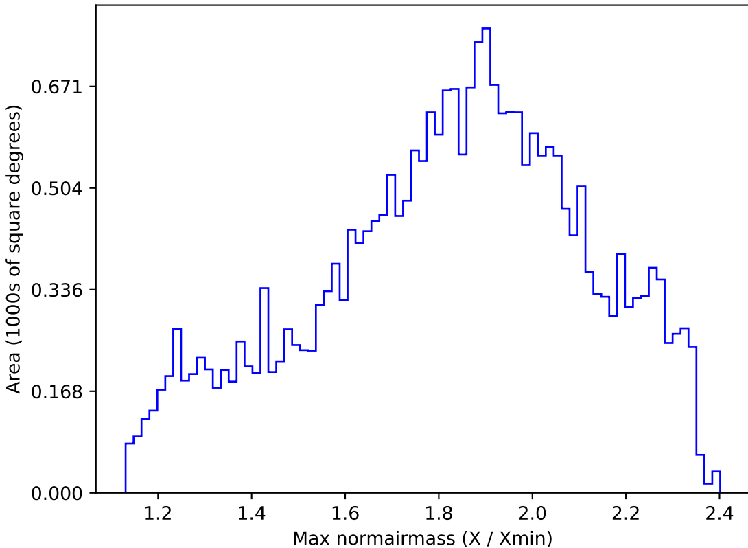
too_100_1v3.4_10yrs All sky g band: Max normairmass
