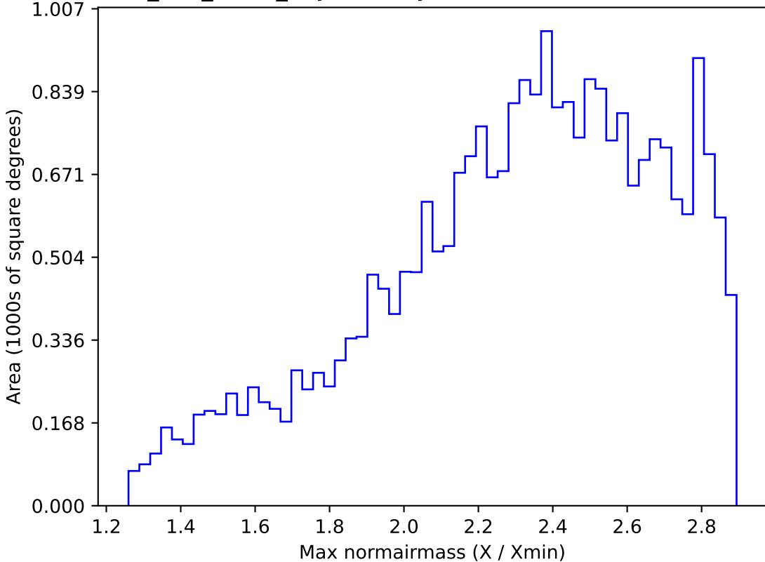
too_100_1v3.4_10yrs All sky all bands: Max normairmass
