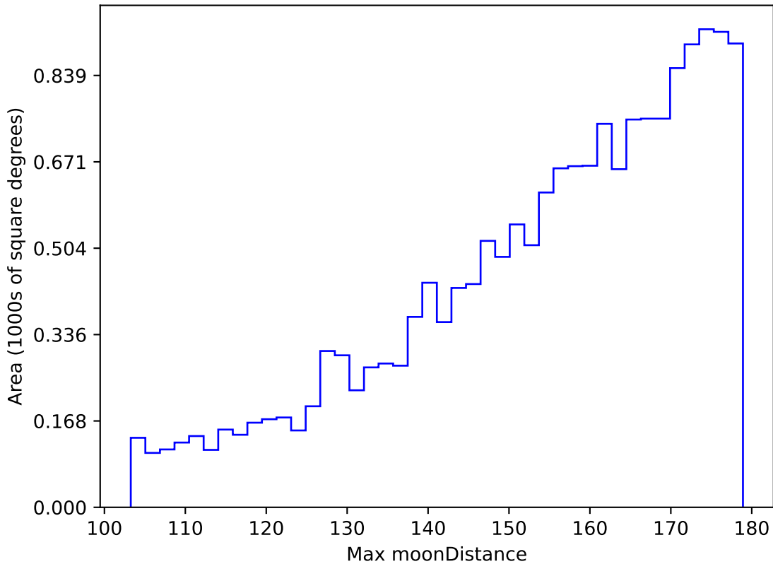
too_100_1v3.4_10yrs WFD z band: Max moonDistance
