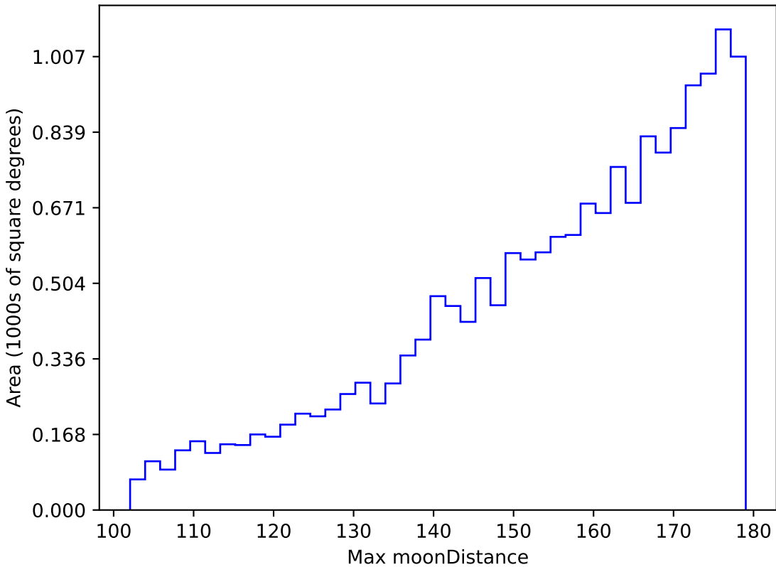
too_100_1v3.4_10yrs WFD u band: Max moonDistance
