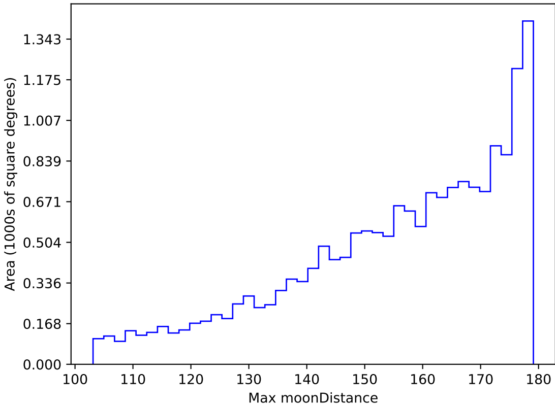
too_100_1v3.4_10yrs WFD i band: Max moonDistance
