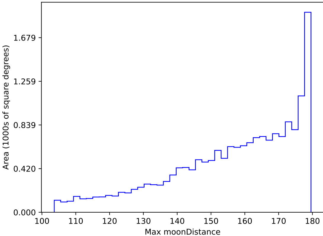
too_100_1v3.4_10yrs WFD all bands: Max moonDistance
