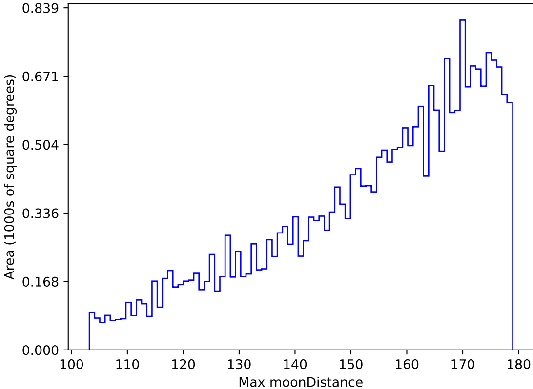
too_100_1v3.4_10yrs All sky z band: Max moonDistance
