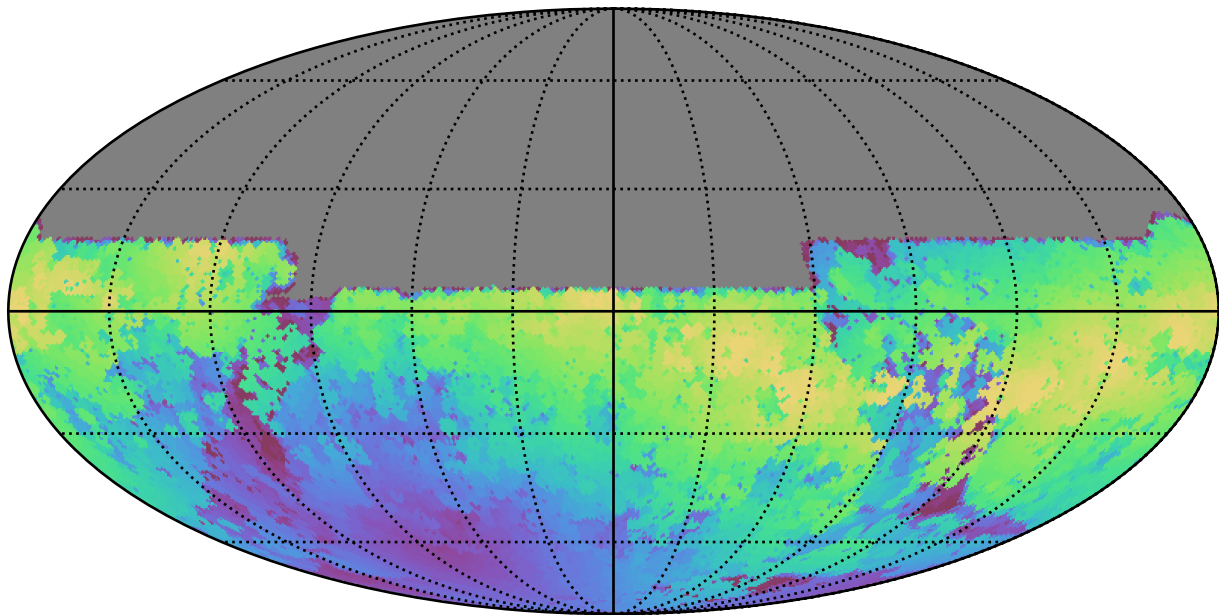
too_100_1v3.4_10yrs All sky y band: Max moonDistance
