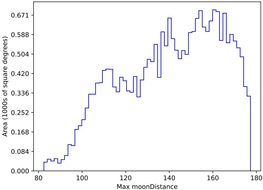
too_100_1v3.4_10yrs All sky y band: Max moonDistance
