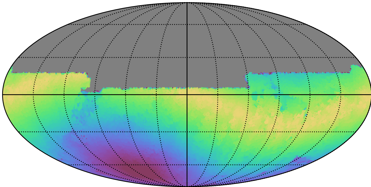
too_100_1v3.4_10yrs All sky u band: Max moonDistance
