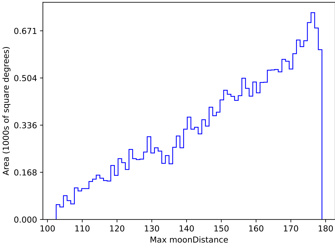
too_100_1v3.4_10yrs All sky u band: Max moonDistance
