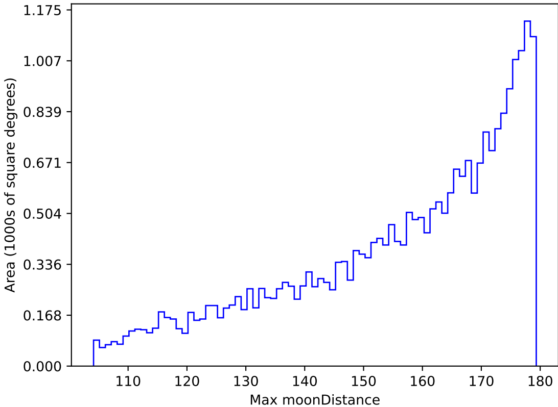
too_100_1v3.4_10yrs All sky r band: Max moonDistance
