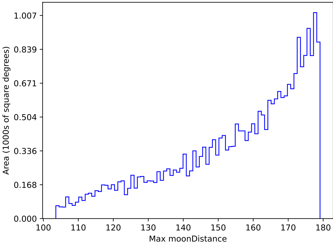
too_100_1v3.4_10yrs All sky i band: Max moonDistance
