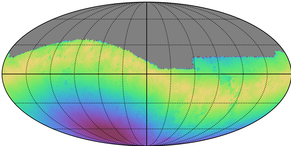
too_100_1v3.4_10yrs All sky g band: Max moonDistance
