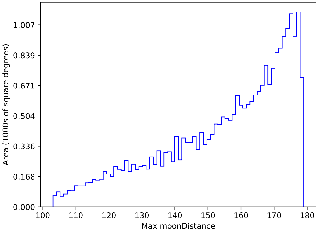
too_100_1v3.4_10yrs All sky g band: Max moonDistance
