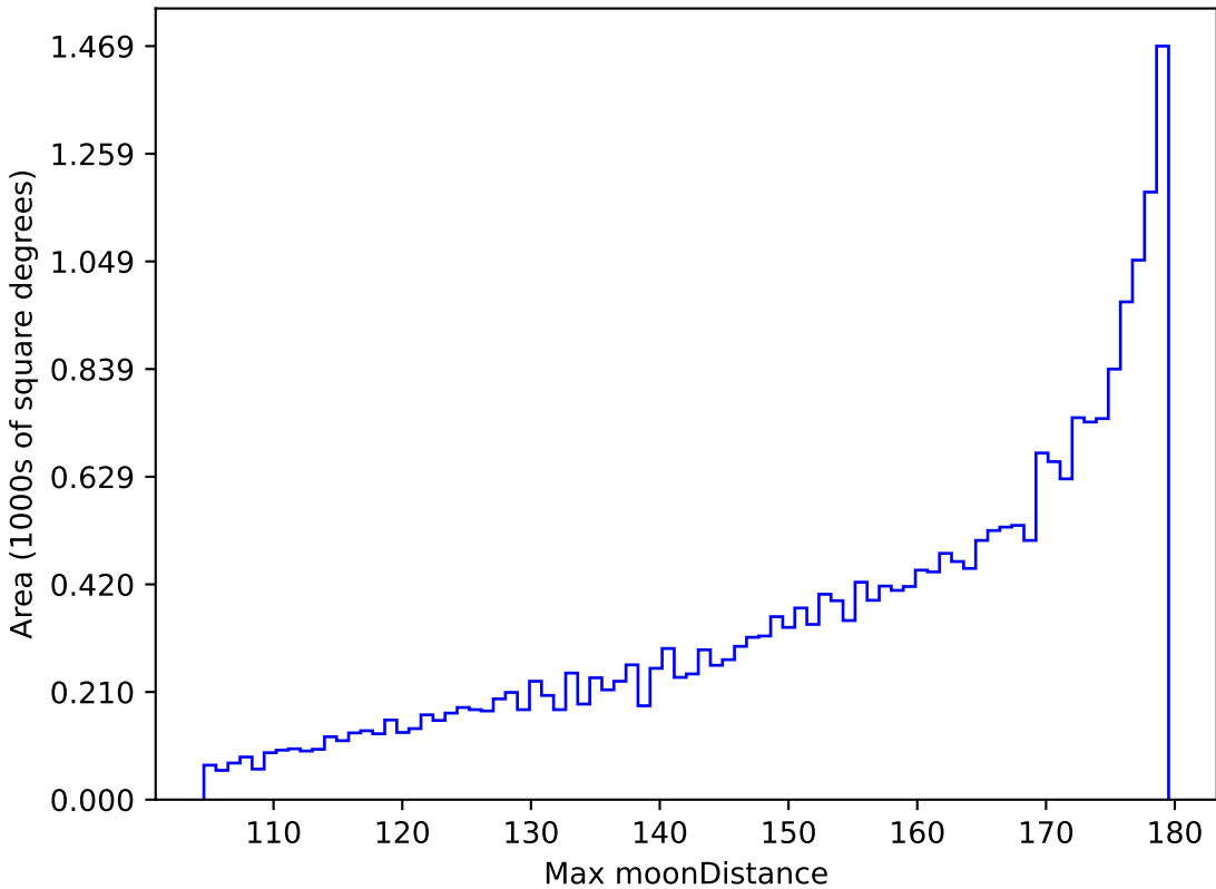
too_100_1v3.4_10yrs All sky all bands: Max moonDistance
