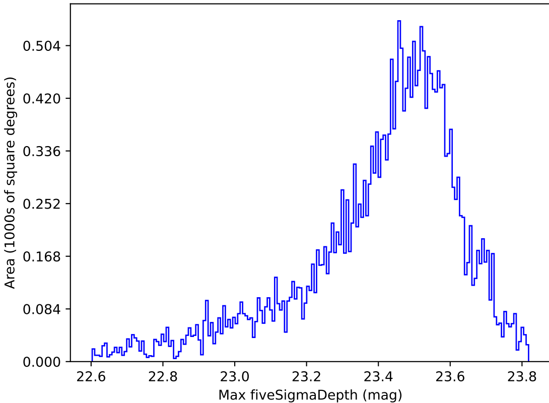
too_100_1v3.4_10yrs Yr 1 z band: Max fiveSigmaDepth
