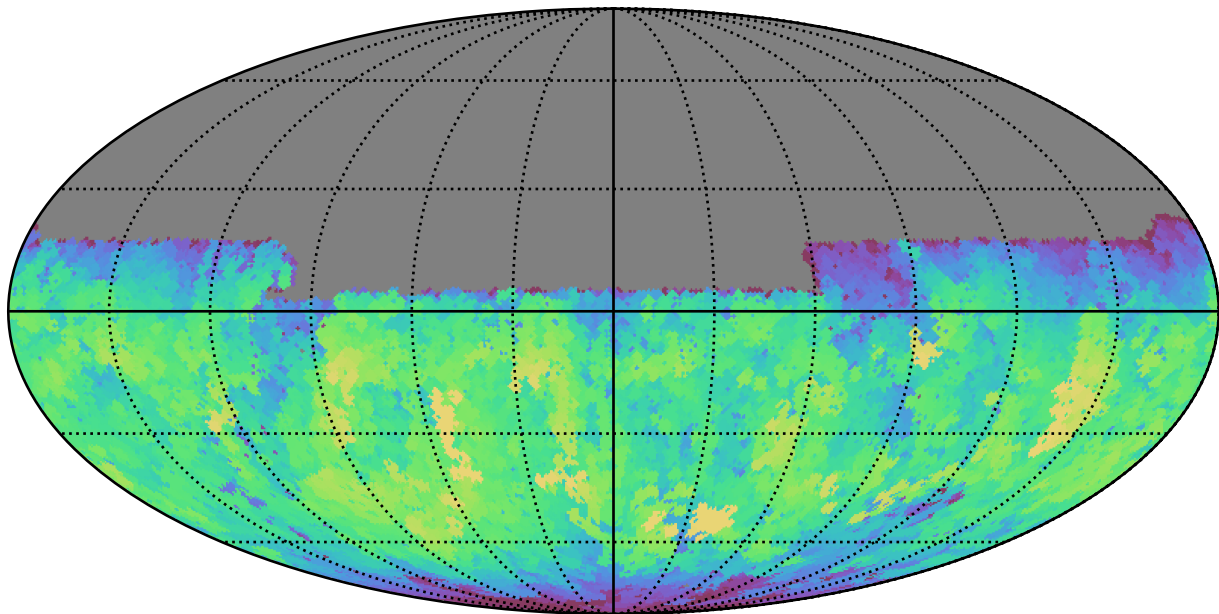
too_100_1v3.4_10yrs Yr 1 y band: Max fiveSigmaDepth
