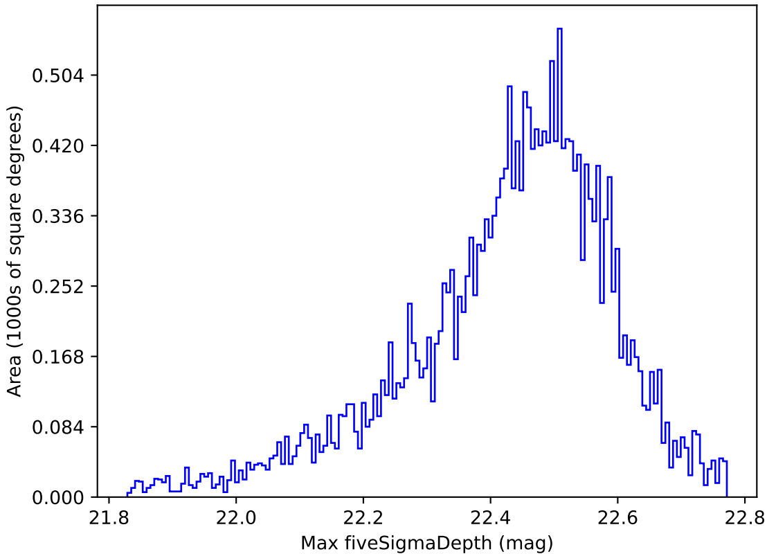
too_100_1v3.4_10yrs Yr 1 y band: Max fiveSigmaDepth
