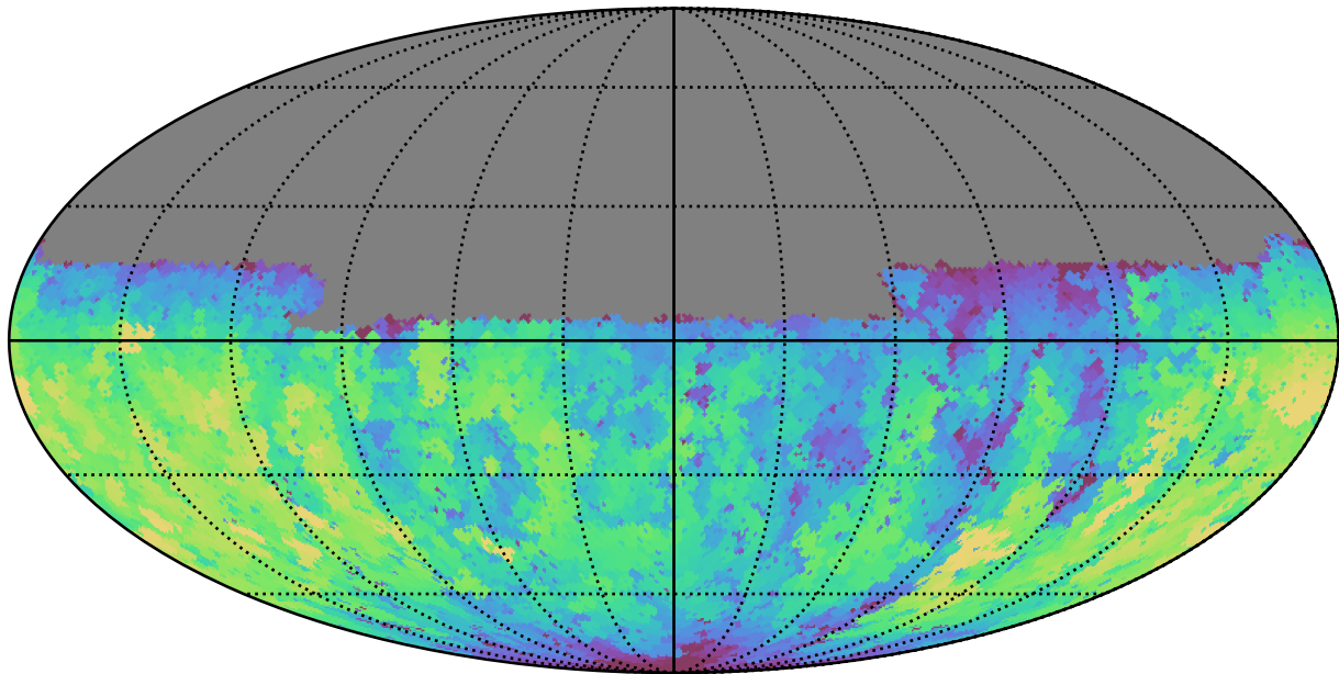
too_100_1v3.4_10yrs Yr 1 u band: Max fiveSigmaDepth
