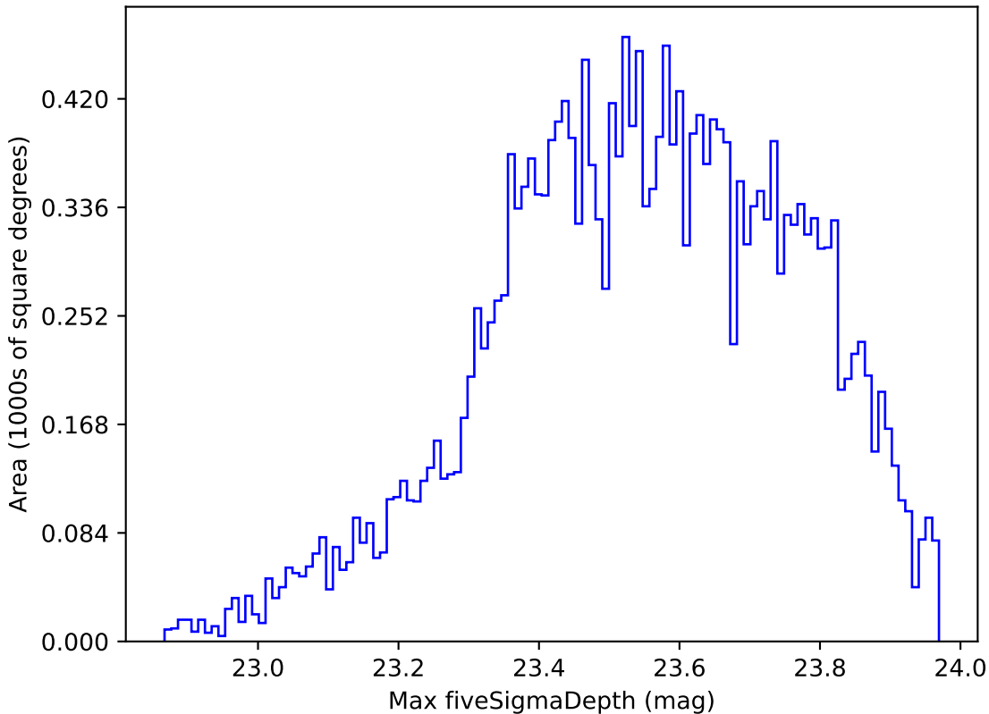
too_100_1v3.4_10yrs Yr 1 u band: Max fiveSigmaDepth
