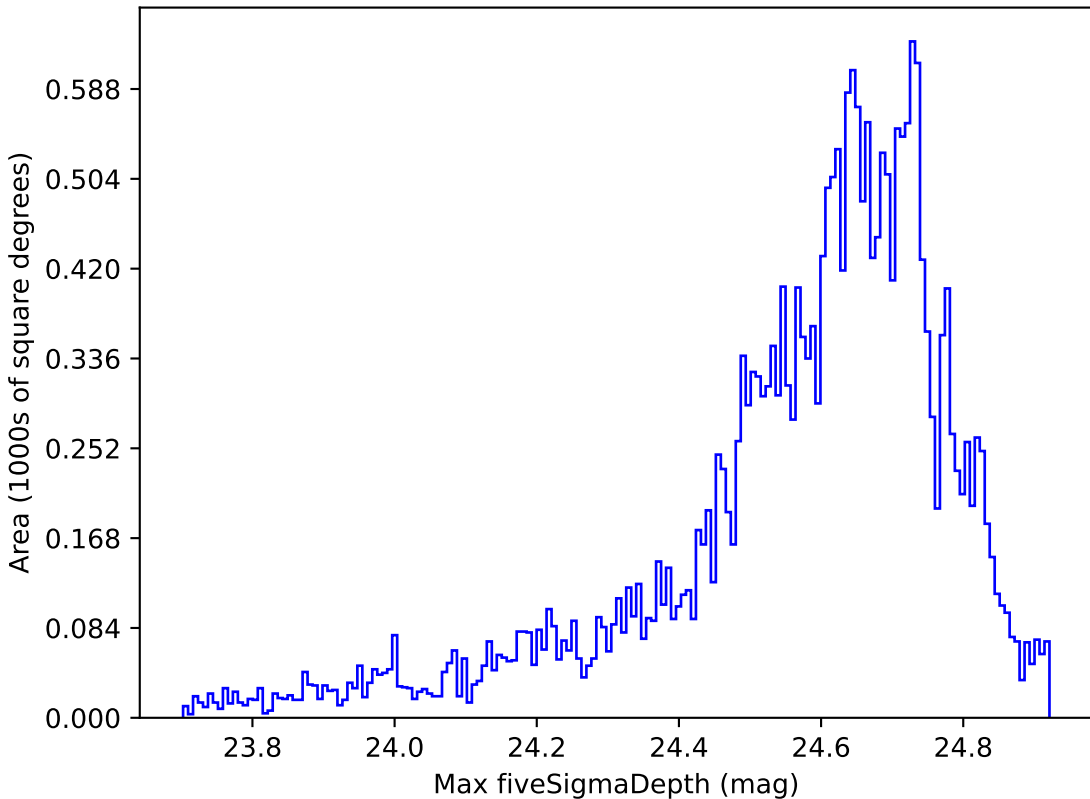
too_100_1v3.4_10yrs Yr 1 r band: Max fiveSigmaDepth
