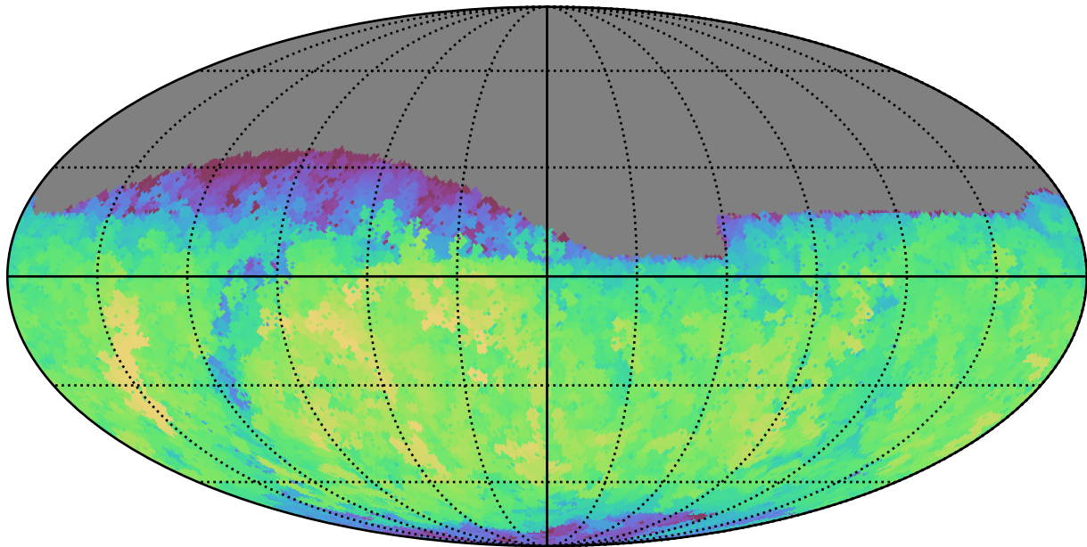
too_100_1v3.4_10yrs Yr 1 i band: Max fiveSigmaDepth
