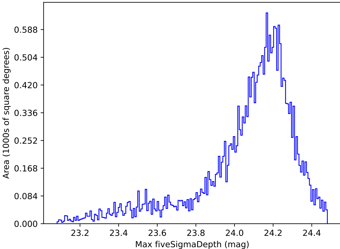
too_100_1v3.4_10yrs Yr 1 i band: Max fiveSigmaDepth
