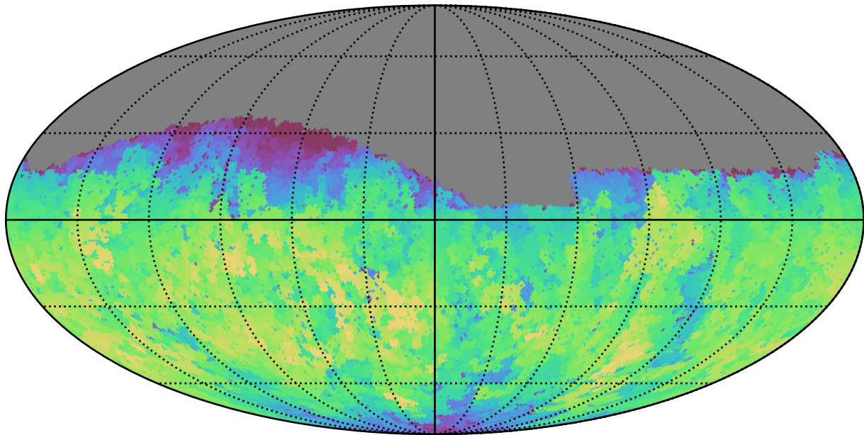
too_100_1v3.4_10yrs Yr 1 g band: Max fiveSigmaDepth
