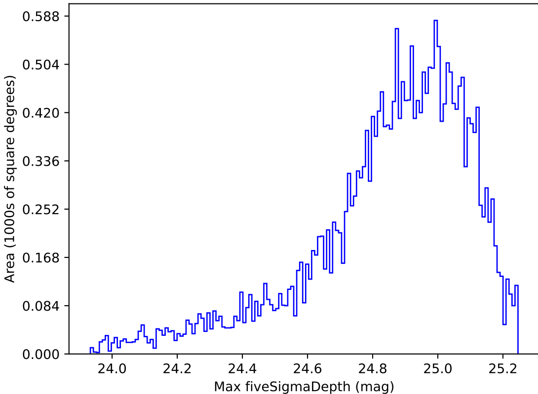
too_100_1v3.4_10yrs Yr 1 g band: Max fiveSigmaDepth
