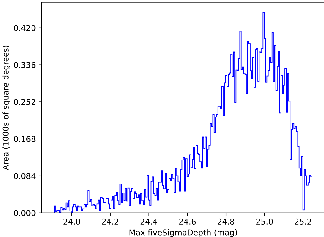
too_100_1v3.4_10yrs Yr 1 all bands: Max fiveSigmaDepth
