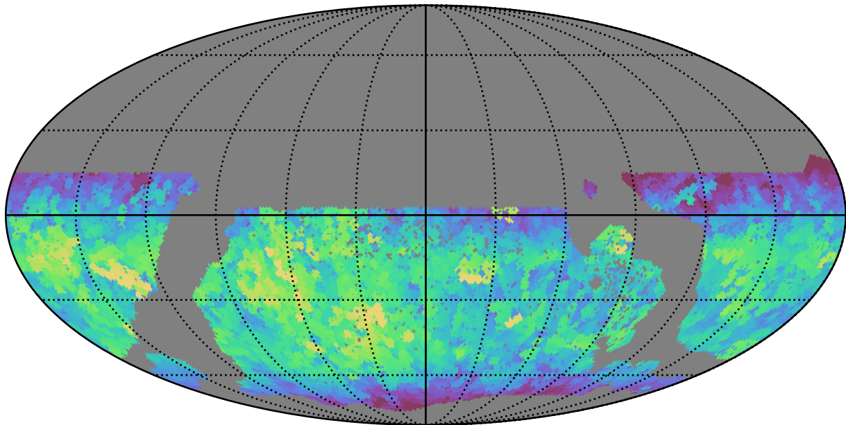
too_100_1v3.4_10yrs WFD z band: Max fiveSigmaDepth
