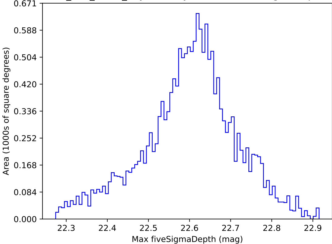
too_100_1v3.4_10yrs WFD y band: Max fiveSigmaDepth
