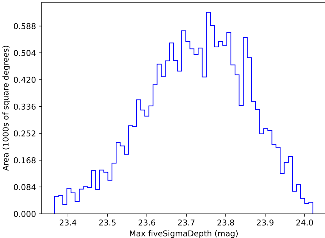
too_100_1v3.4_10yrs WFD u band: Max fiveSigmaDepth
